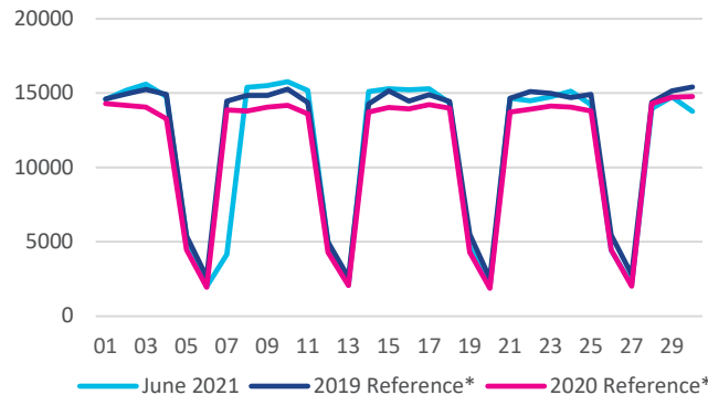
M50 J4 - J5 HGV 24H Flow
