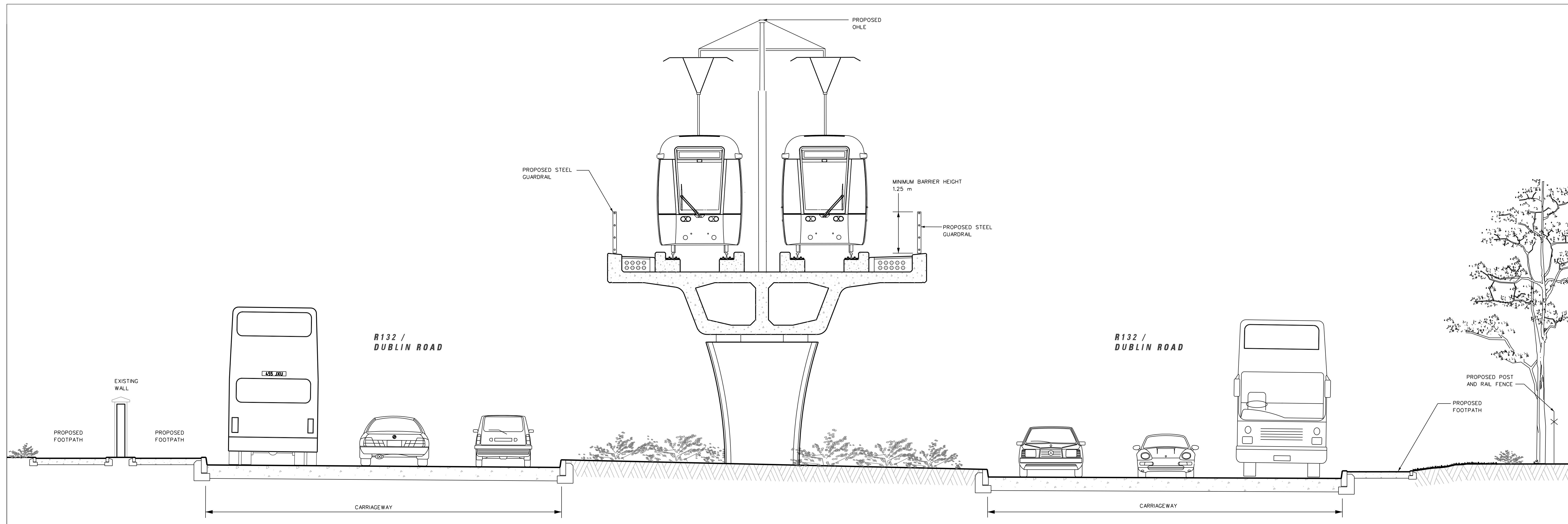
SECTIONAL ELEVATION B-B SCALE 1:50
