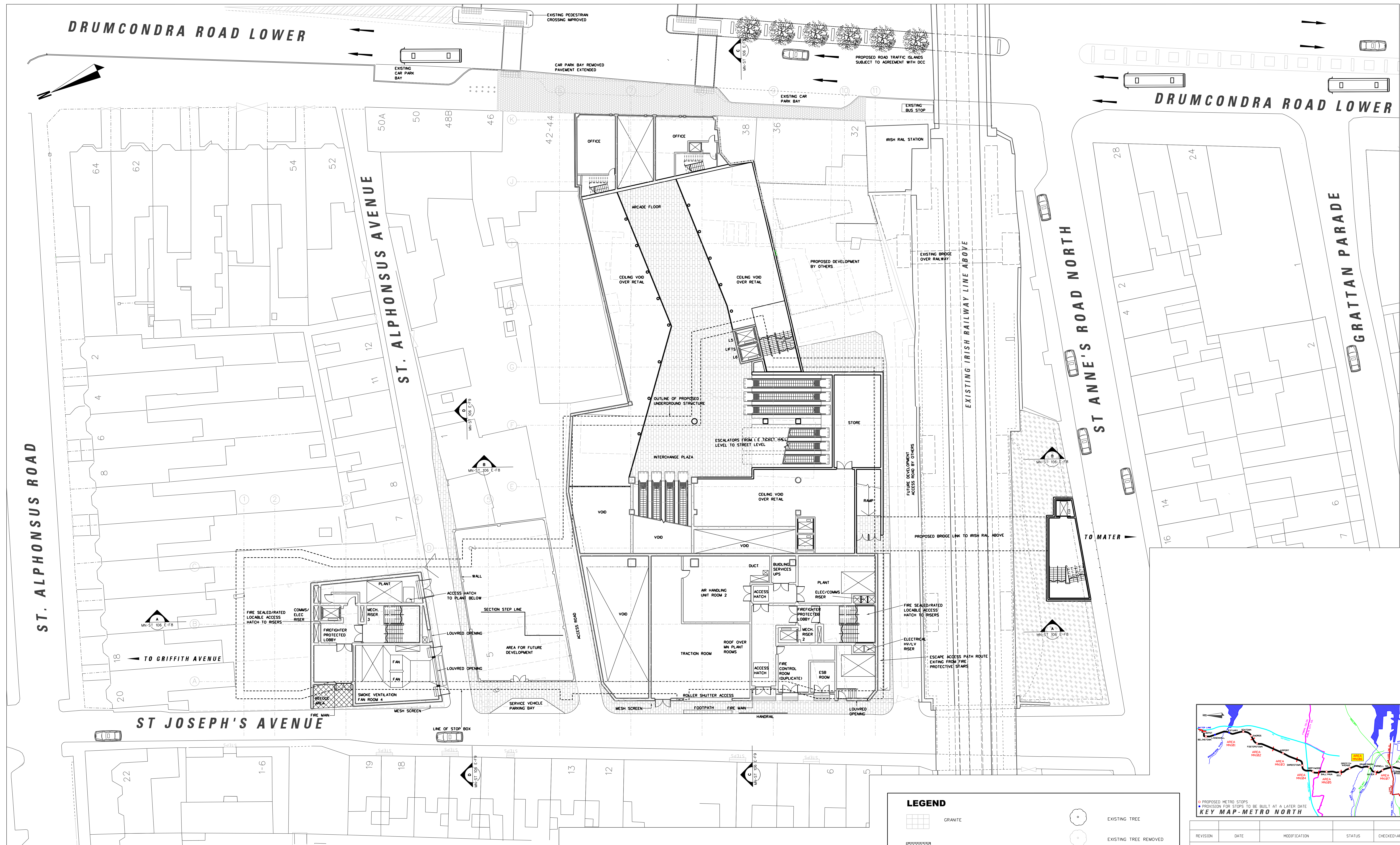
STREET LEVEL PLAN (ST JOSEPH'S AVENUE) SCALE 1:200
