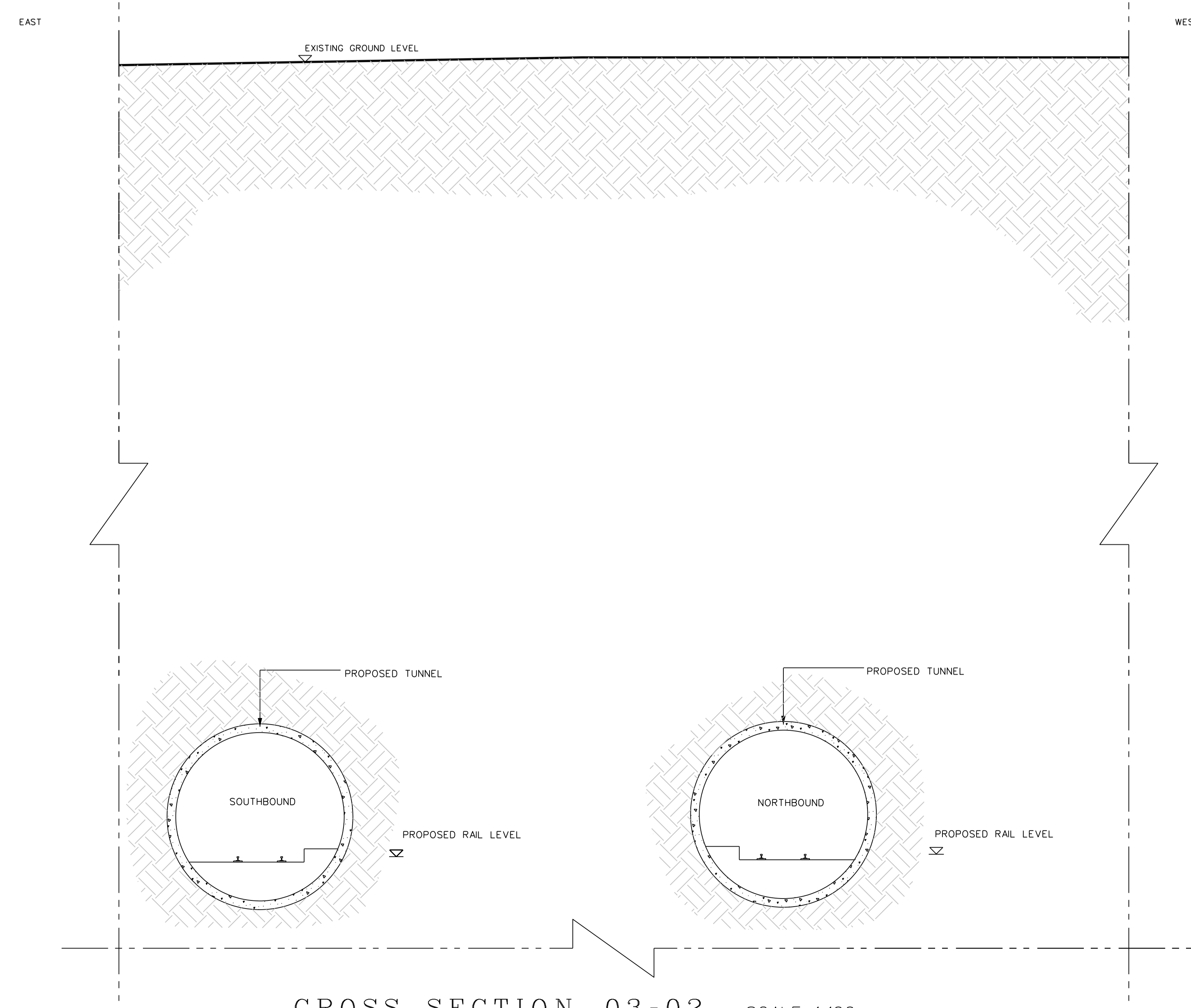
CROSS SECTION 03-02 SCALE 1:100
