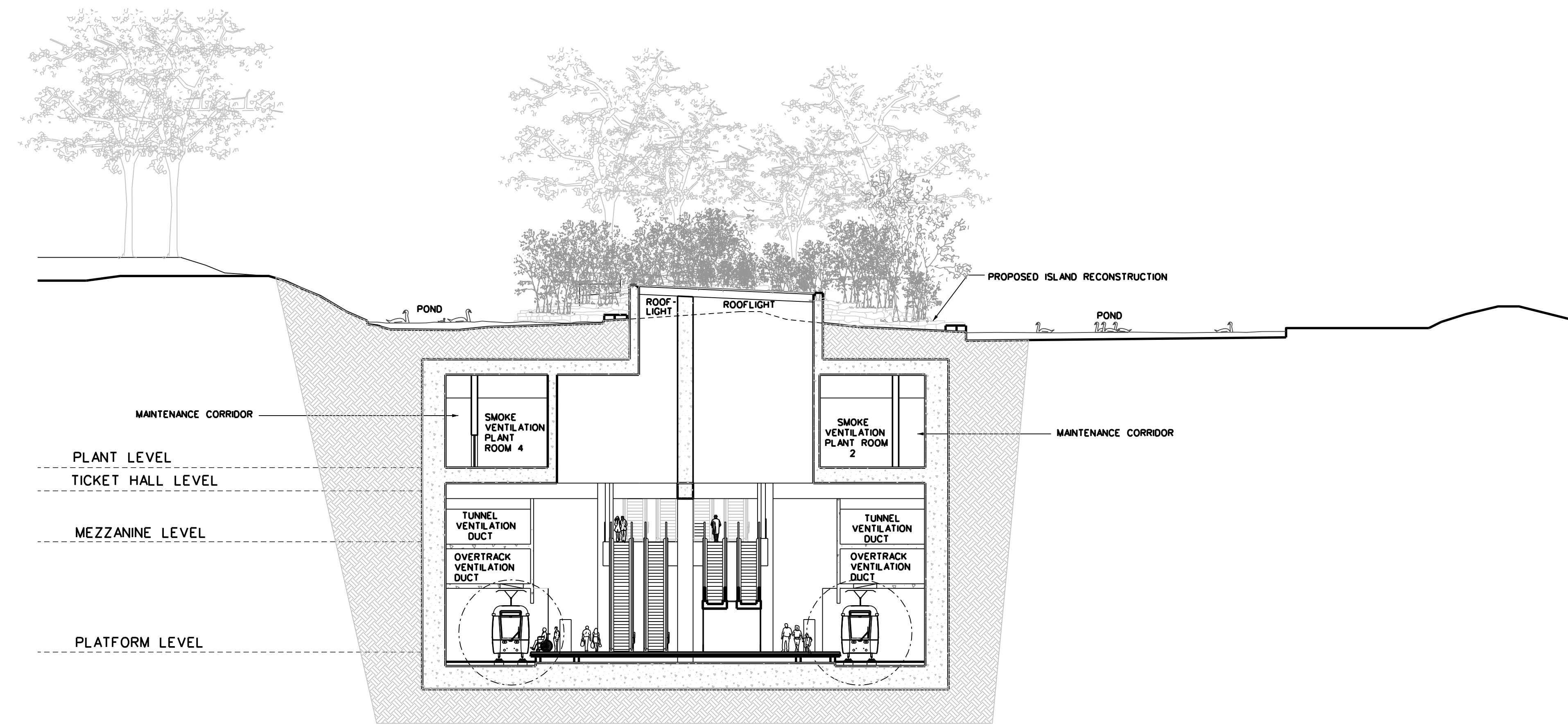
SECTION D-D SCALE 1:200
