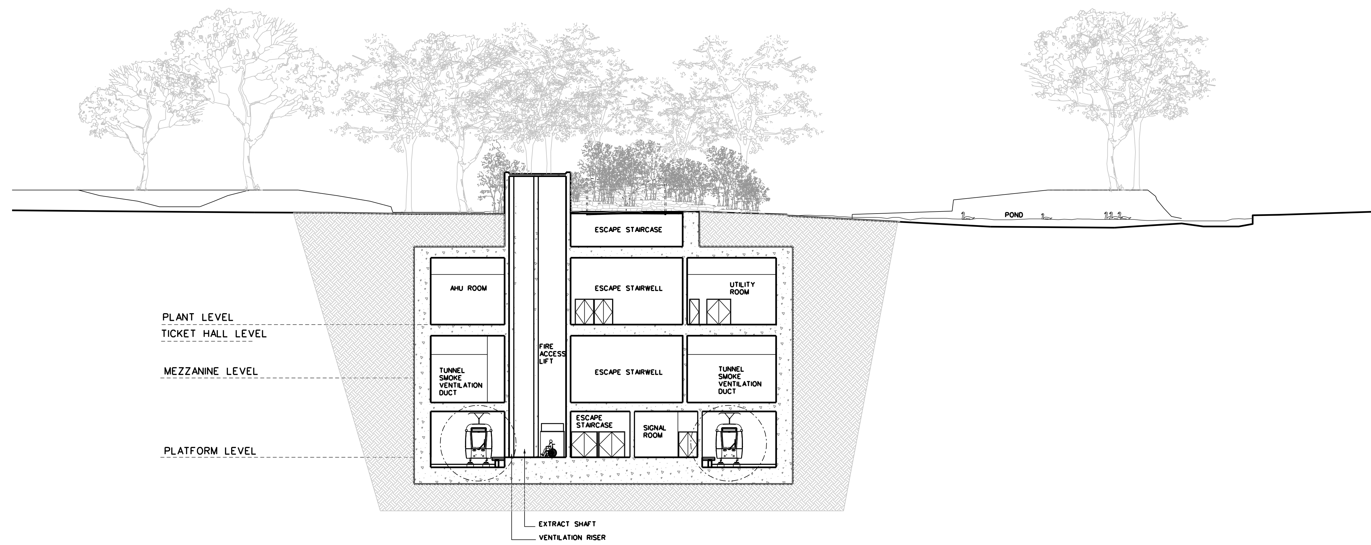
SECTION C-C SCALE 1:200
