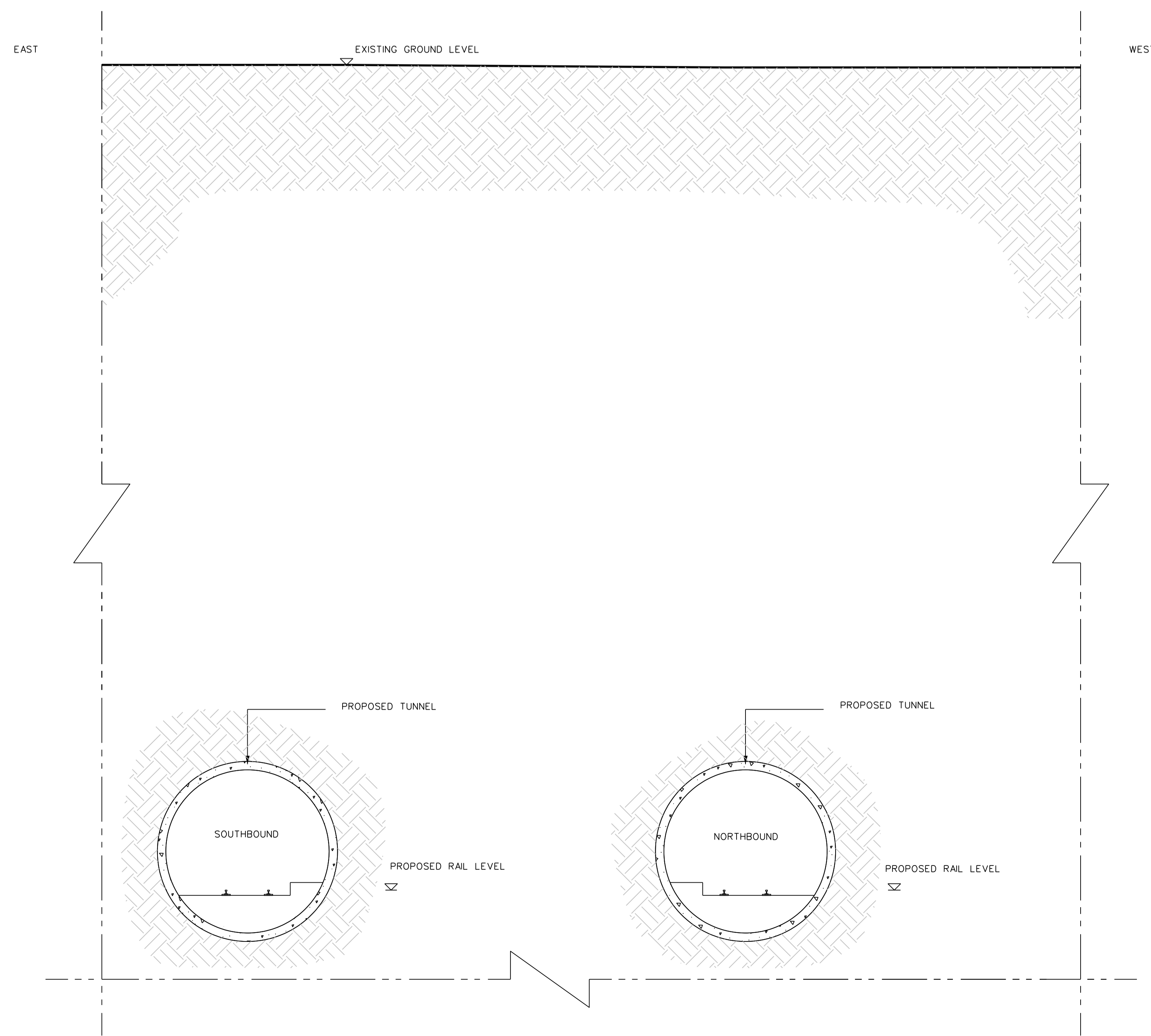
CROSS SECTION 03-04 SCALE 1:100
