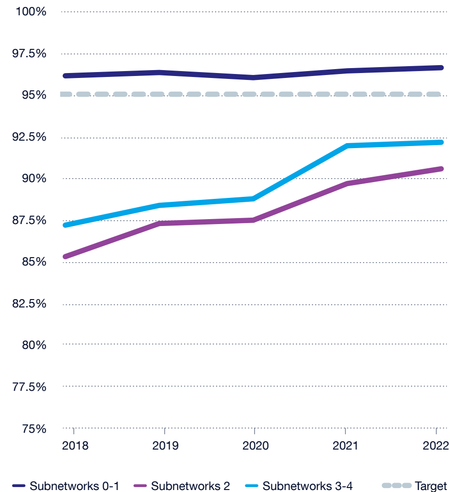
Trends in Pavement Surface Health KPI* (% Fair or Better) (2018-2022)
