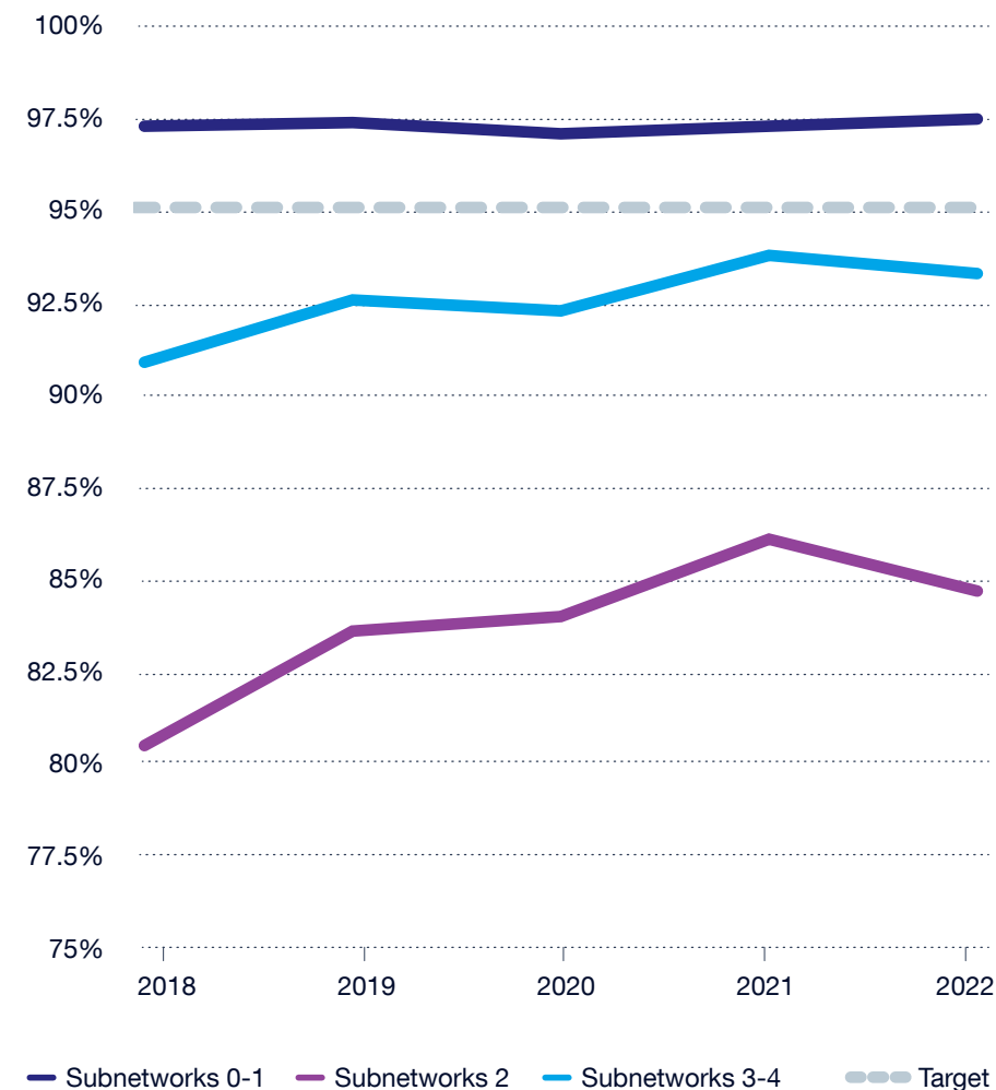
Trends in Pavement Structural Health KPI* (% Fair or Better) (2018-2022)
