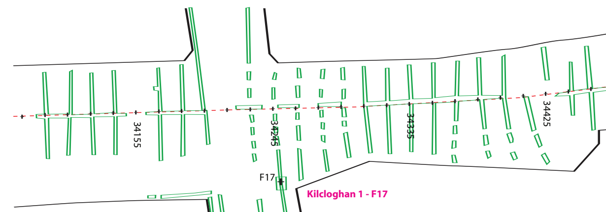
Plan of continuous and collinear test-trenches in an area of reclaimed peatland along the route of the N6 Kinnegad to Kilbeggan Road Scheme. (Cultural Resource Development Services Ltd.)
