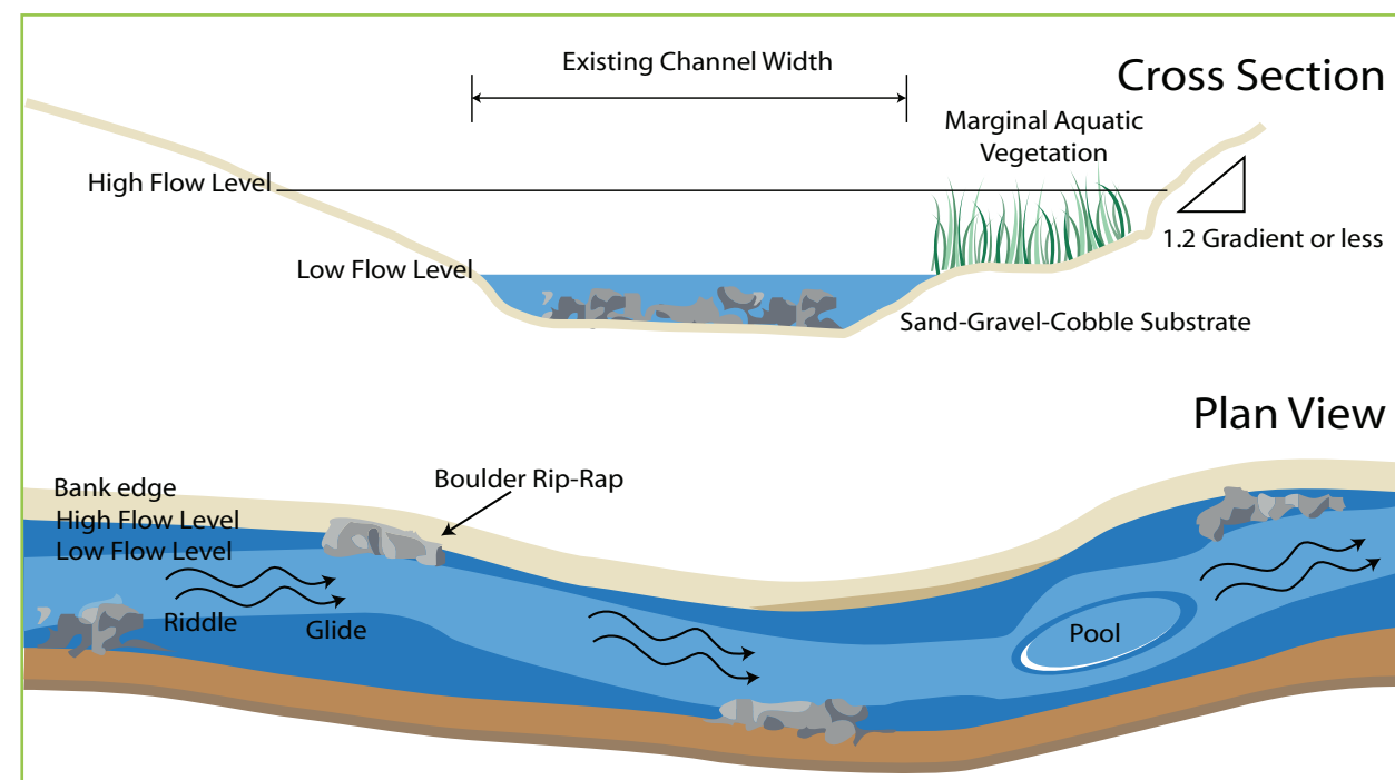
FIGURE 1 A schematic drawing of a section of realigned watercourse channel showing the necessary features to be incorporated, including meanders, variation in flow regime and gently profiled banks which will allow for the establishment of a native riparian and aquatic marginal vegetation and to allow access to the stream bed for wildlife.
