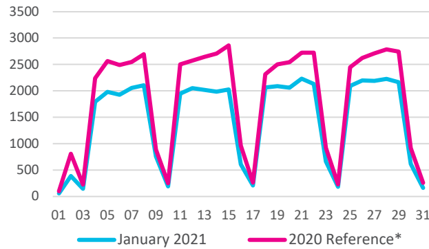
M50 J3 - J4 HGV AM Flow
