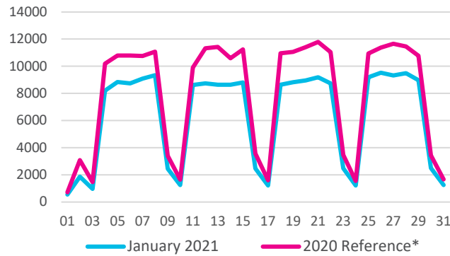
M50 J3 - J4 HGV 24H Flow
