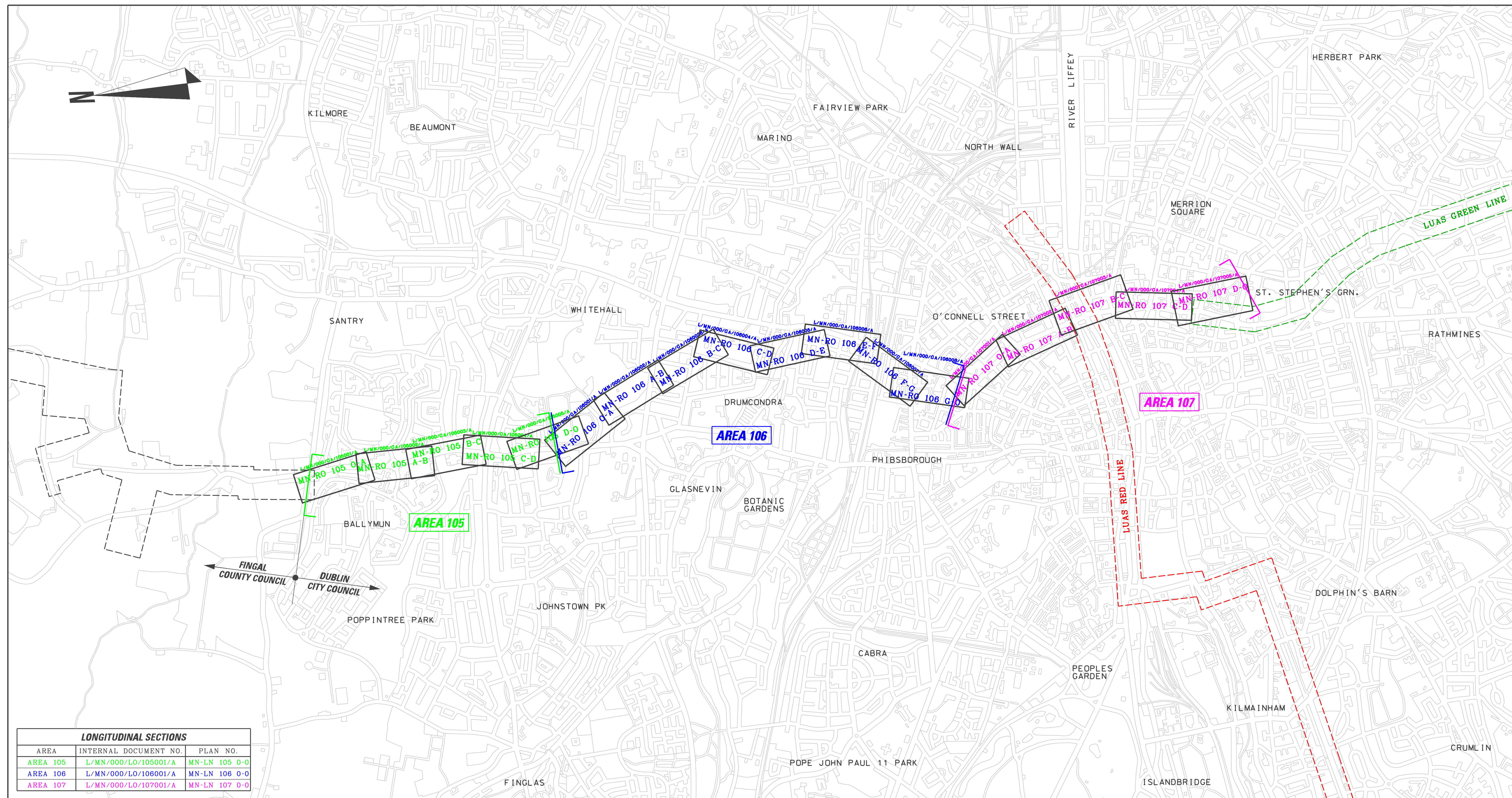
KEY MAP LAYOUT - ALIGNMENT
