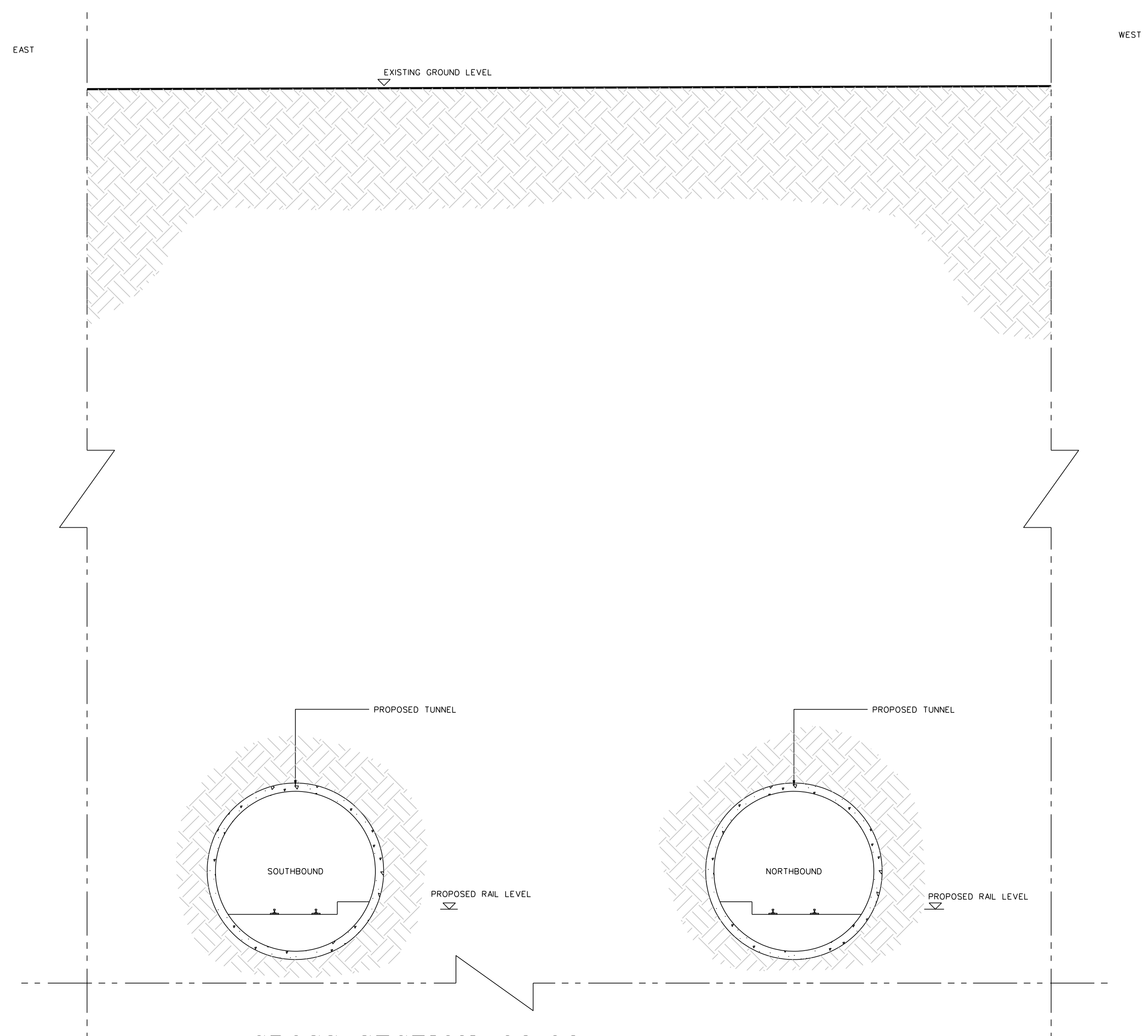
CROSS SECTION 06-06 SCALE 1:100
