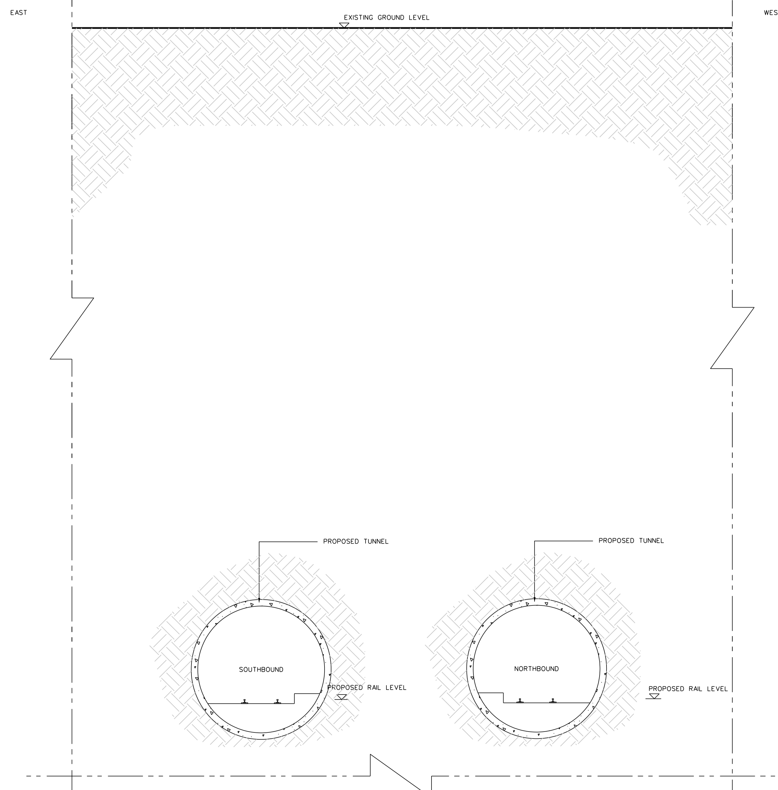
CROSS SECTION 07-01 SCALE 1:100
