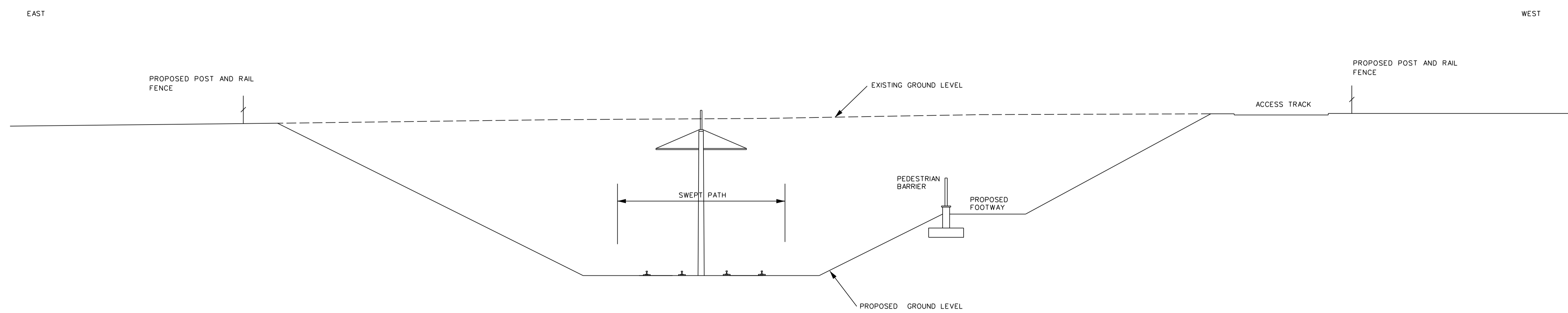
CROSS SECTION 02-03 SCALE 1:100
