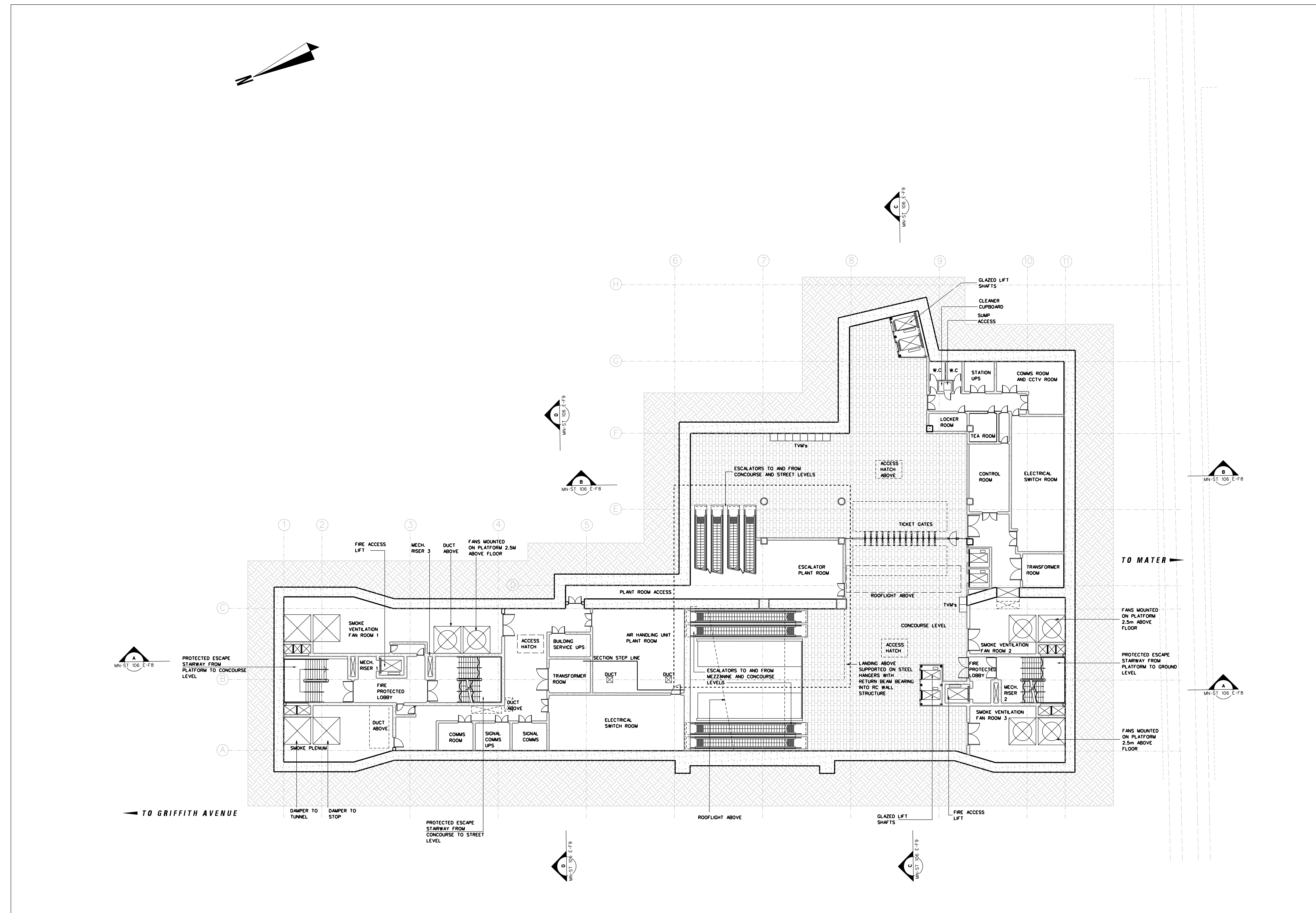
CONCOURSE LEVEL PLAN SCALE 1:200
