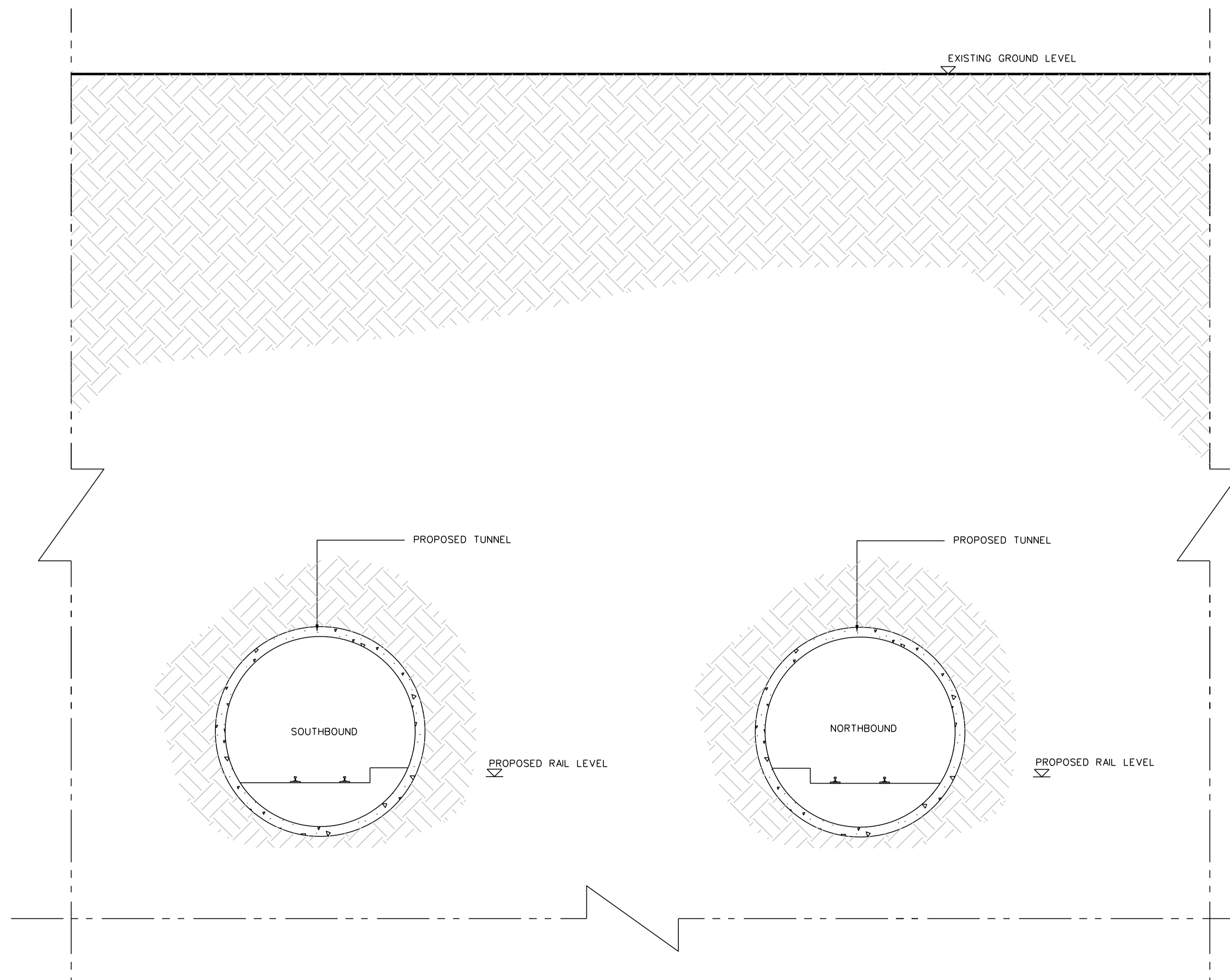
CROSS SECTION 03-03 SCALE 1:100
